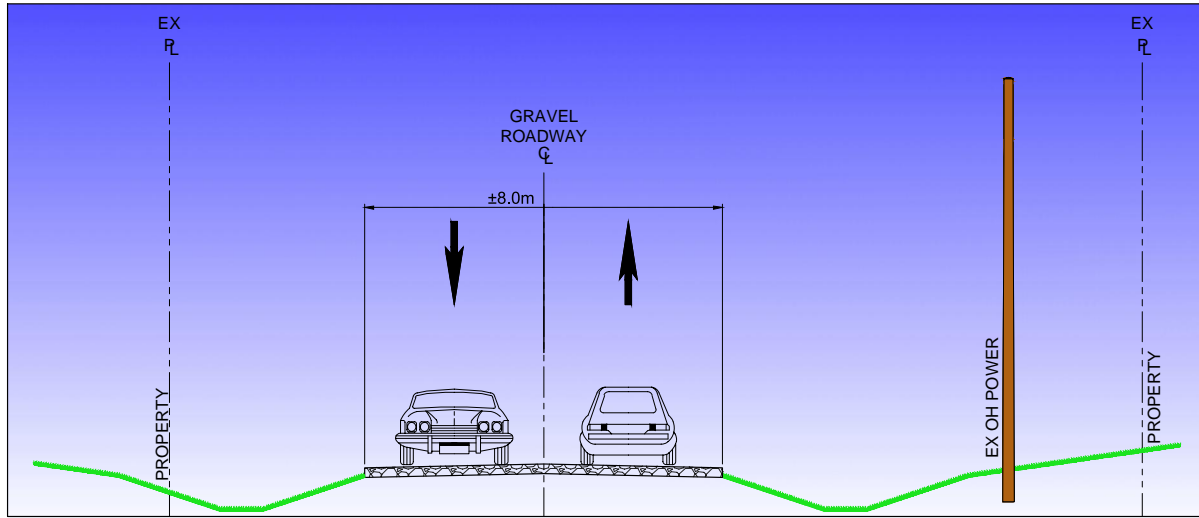
PROPOSED CROSS SECTION
